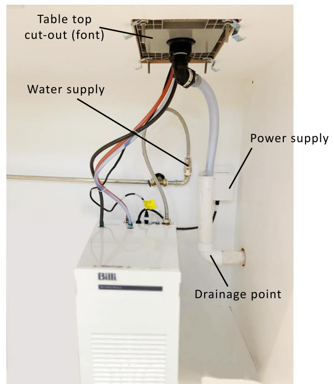
Optional - drainage point with bottle trap (connection to be completed by your contractor)
